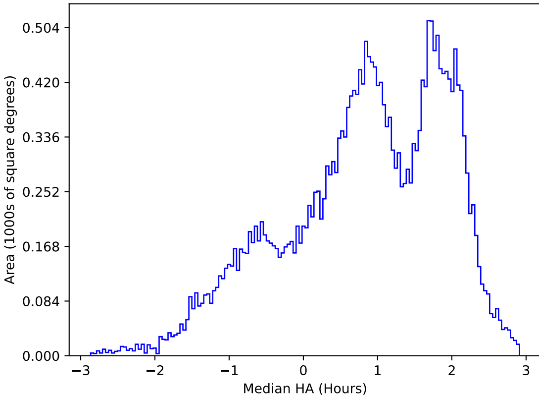
weather_cloudso36v3.4_10yrs All sky i band: Median HA
