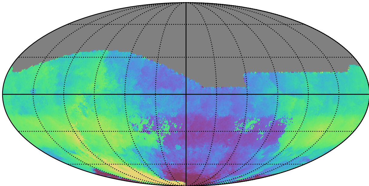
weather_cloudso36v3.4_10yrs All sky g band: Median HA
