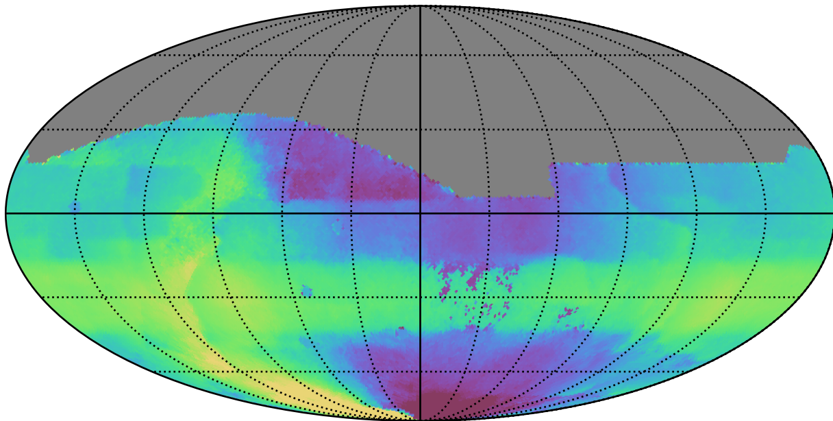
weather_cloudso36v3.4_10yrs All sky all bands: Median HA
