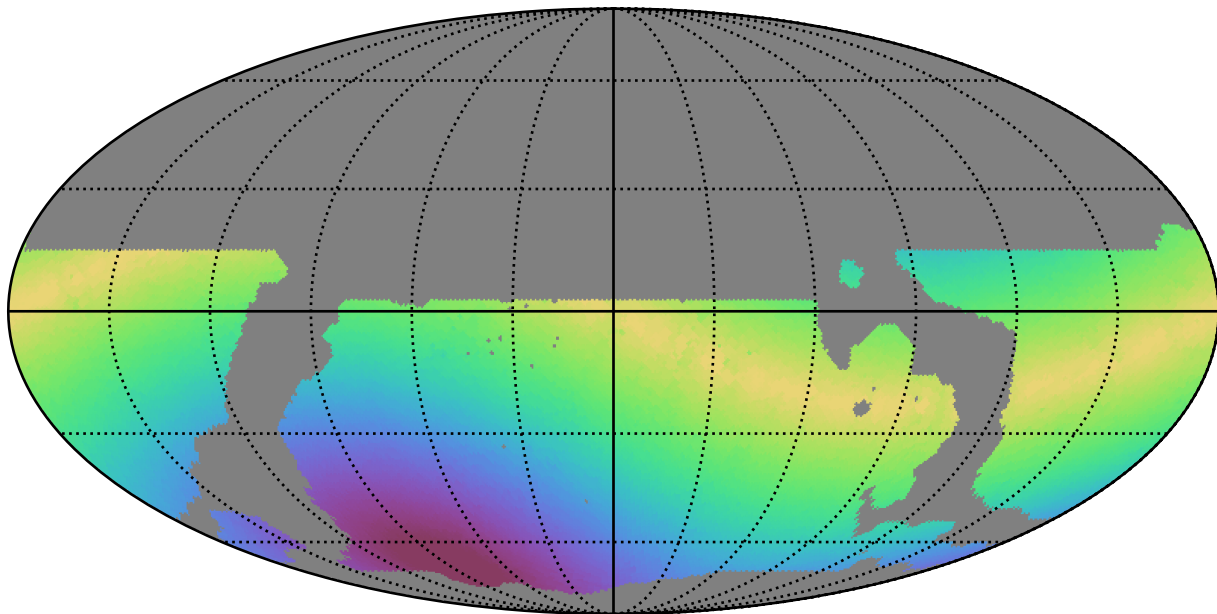
weather_cloudso36v3.4_10yrs WFD u band: Max solarElong
