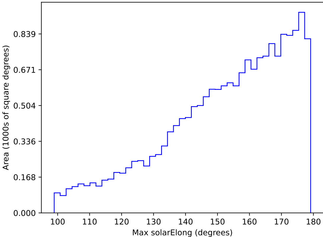
weather_cloudso36v3.4_10yrs WFD u band: Max solarElong
