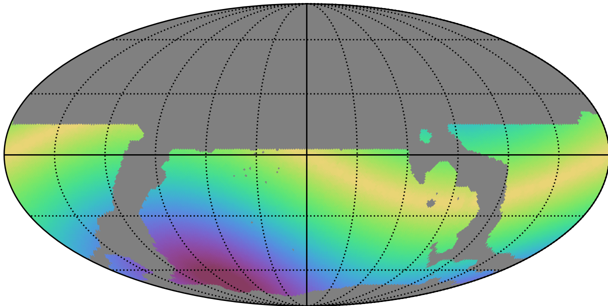
weather_cloudso36v3.4_10yrs WFD all bands: Max solarElong
