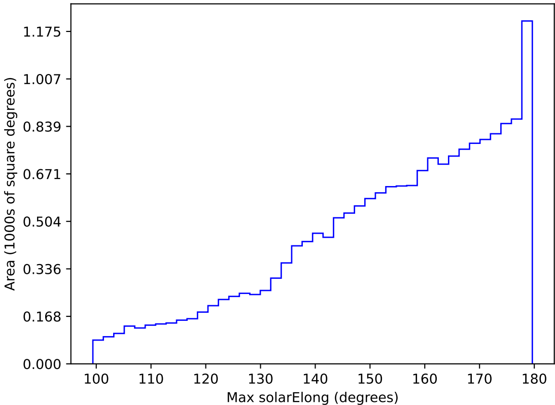
weather_cloudso36v3.4_10yrs WFD all bands: Max solarElong
