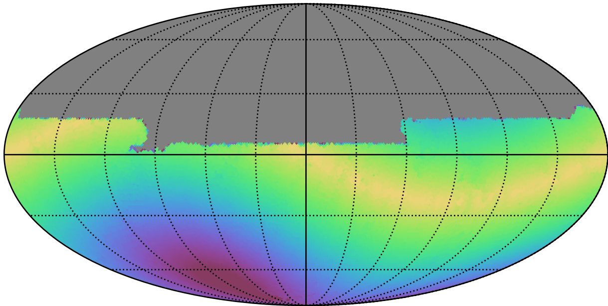
weather_cloudso36v3.4_10yrs All sky u band: Max solarElong
