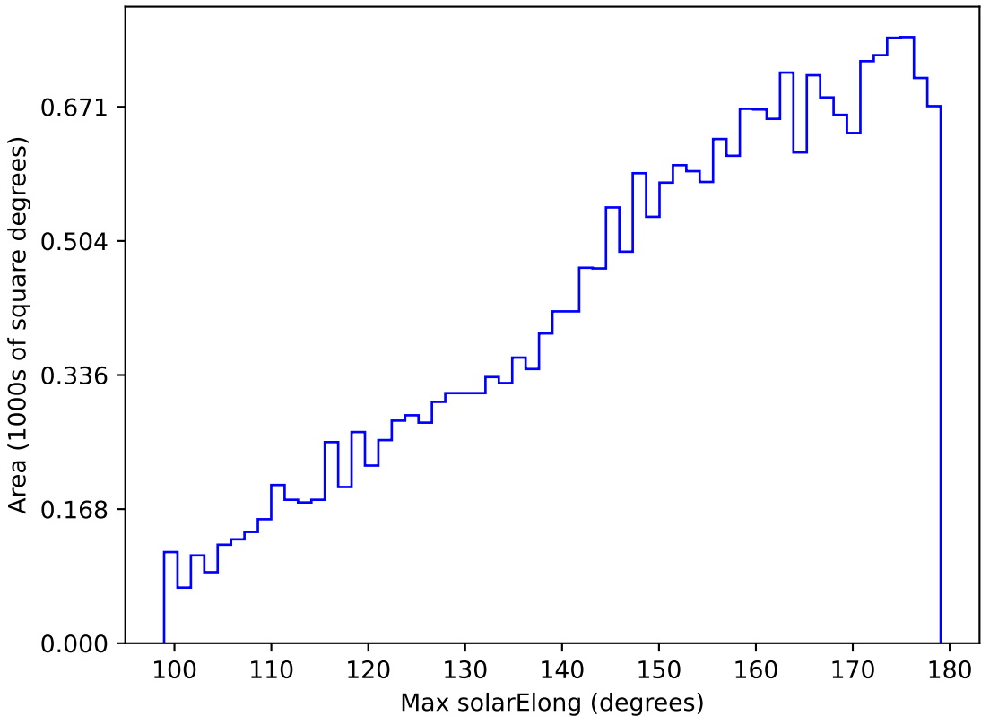
weather_cloudso36v3.4_10yrs All sky u band: Max solarElong
