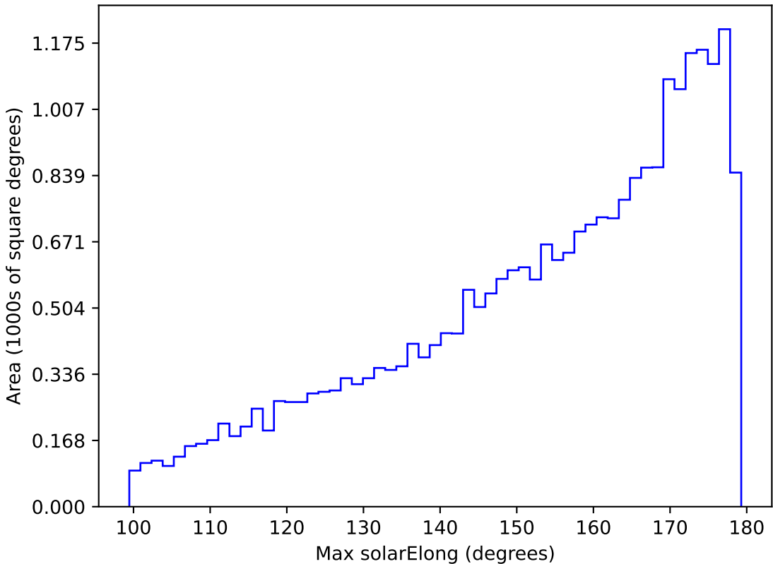
weather_cloudso36v3.4_10yrs All sky g band: Max solarElong
