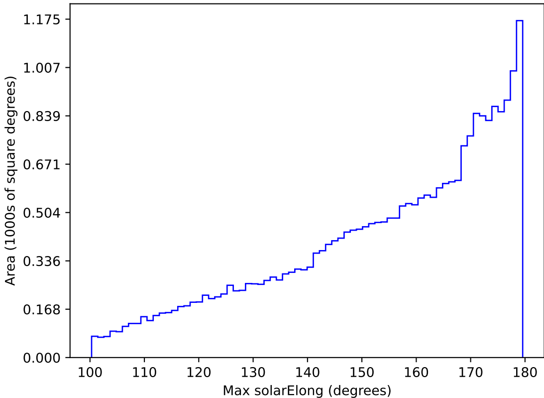
weather_cloudso36v3.4_10yrs All sky all bands: Max solarElong
