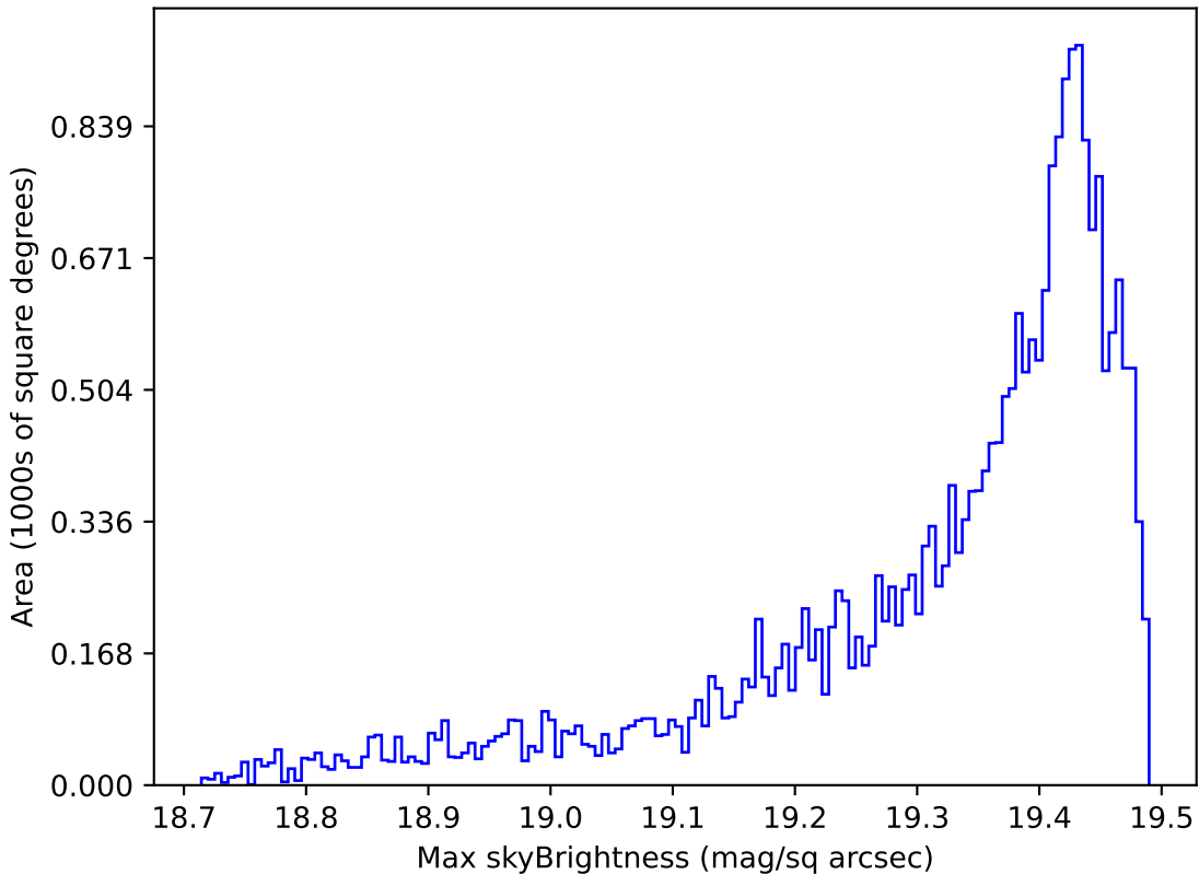
weather_cloudso36v3.4_10yrs Yr 1 z band: Max skyBrightness
