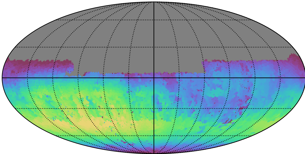
weather_cloudso36v3.4_10yrs Yr 1 u band: Max skyBrightness
