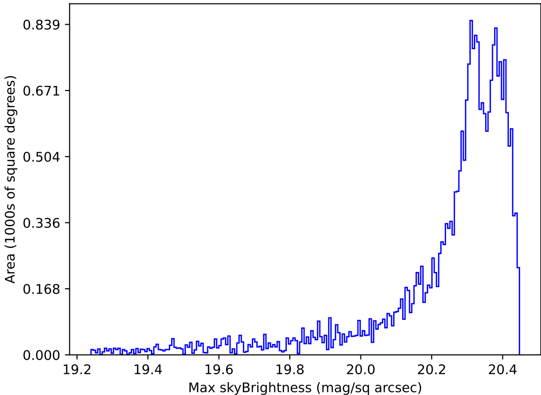
weather_cloudso36v3.4_10yrs Yr 1 i band: Max skyBrightness
