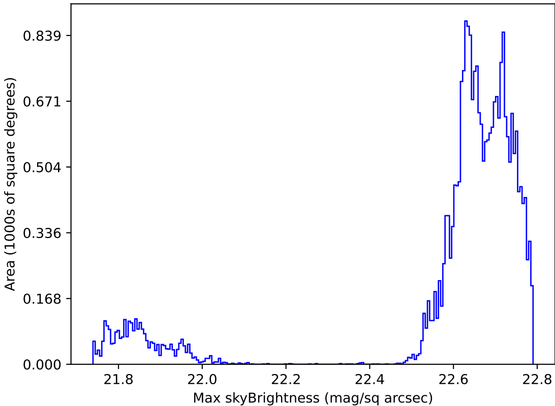
weather_cloudso36v3.4_10yrs Yr 1 all bands: Max skyBrightness
