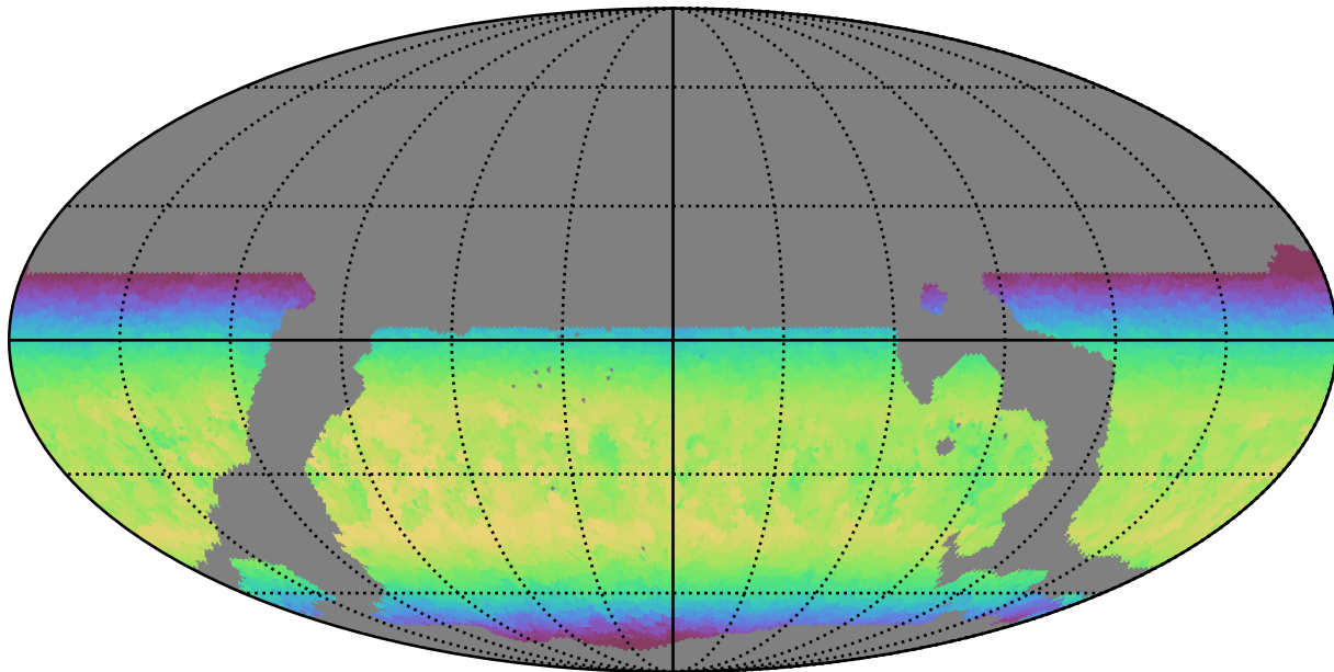
weather_cloudso36v3.4_10yrs WFD y band: Max skyBrightness
