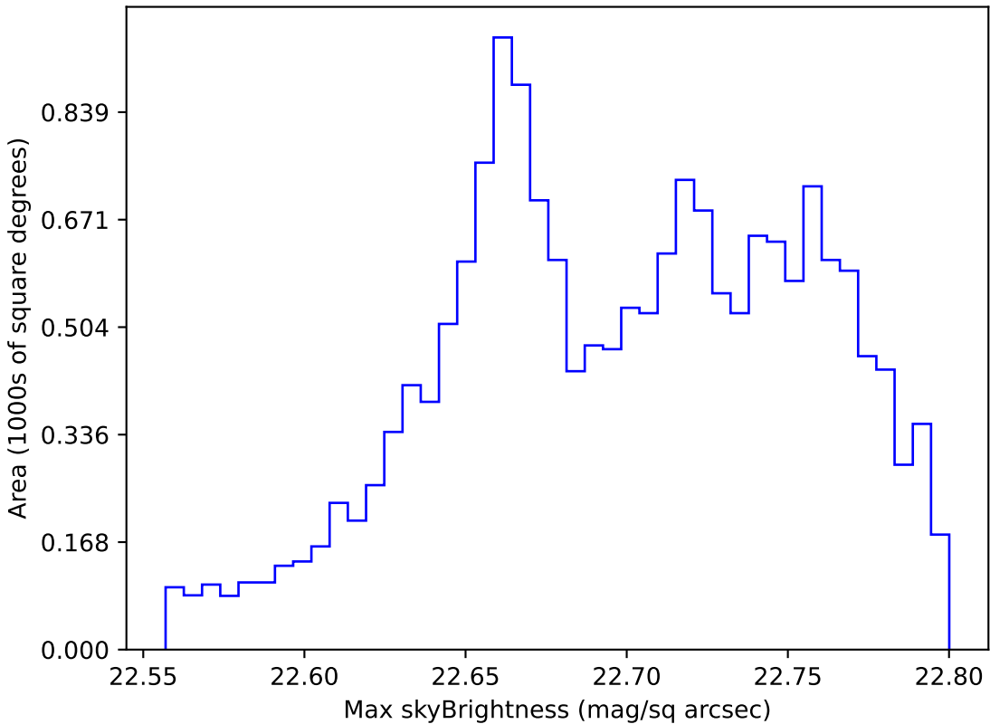
weather_cloudso36v3.4_10yrs WFD u band: Max skyBrightness
