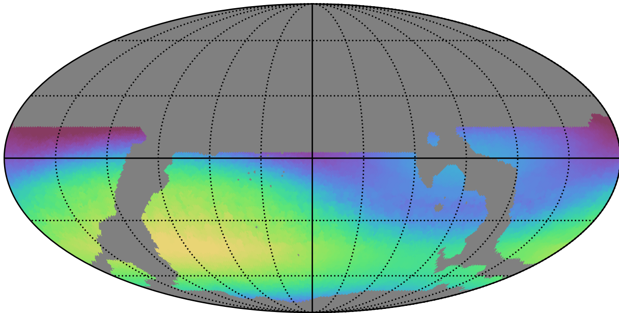
weather_cloudso36v3.4_10yrs WFD r band: Max skyBrightness
