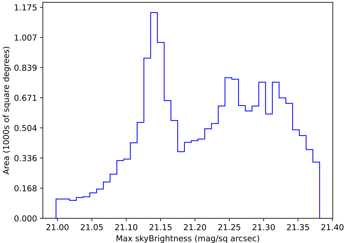
weather_cloudso36v3.4_10yrs WFD r band: Max skyBrightness
