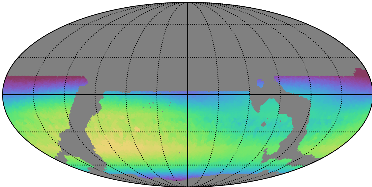
weather_cloudso36v3.4_10yrs WFD i band: Max skyBrightness
