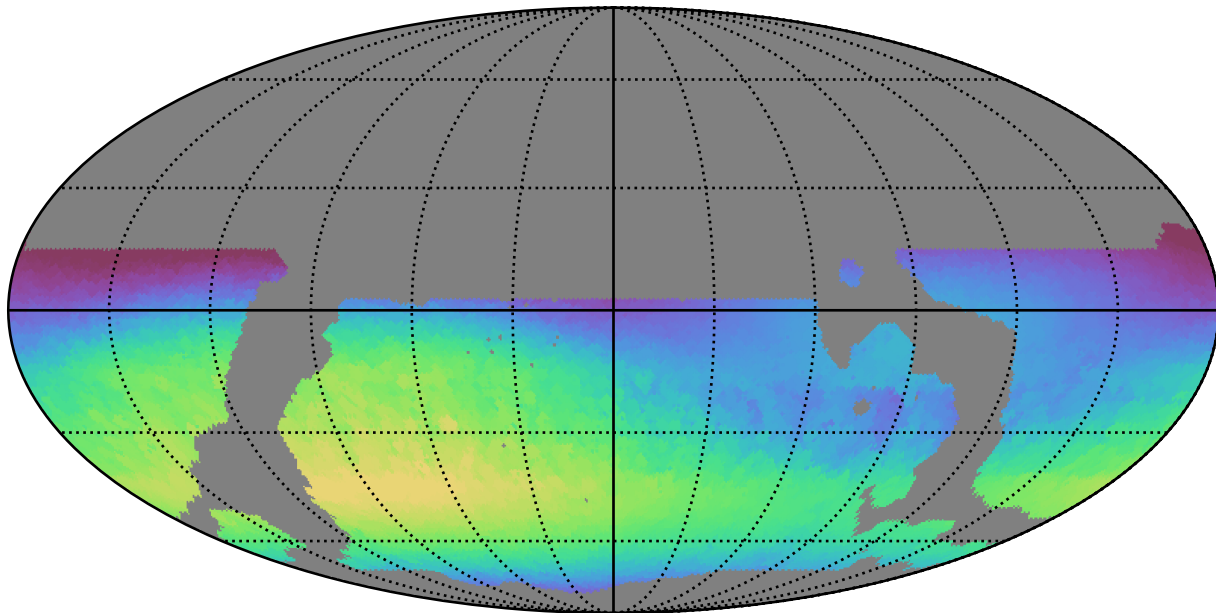
weather_cloudso36v3.4_10yrs WFD all bands: Max skyBrightness
