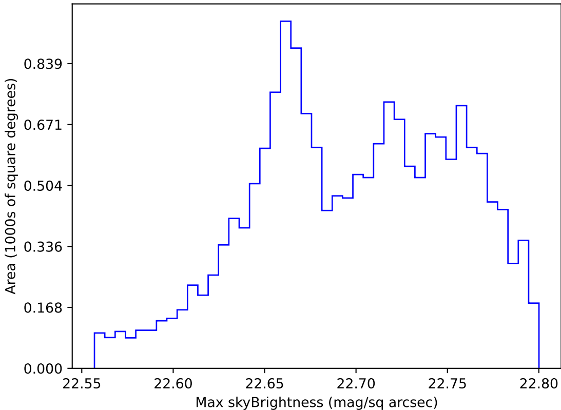
weather_cloudso36v3.4_10yrs WFD all bands: Max skyBrightness
