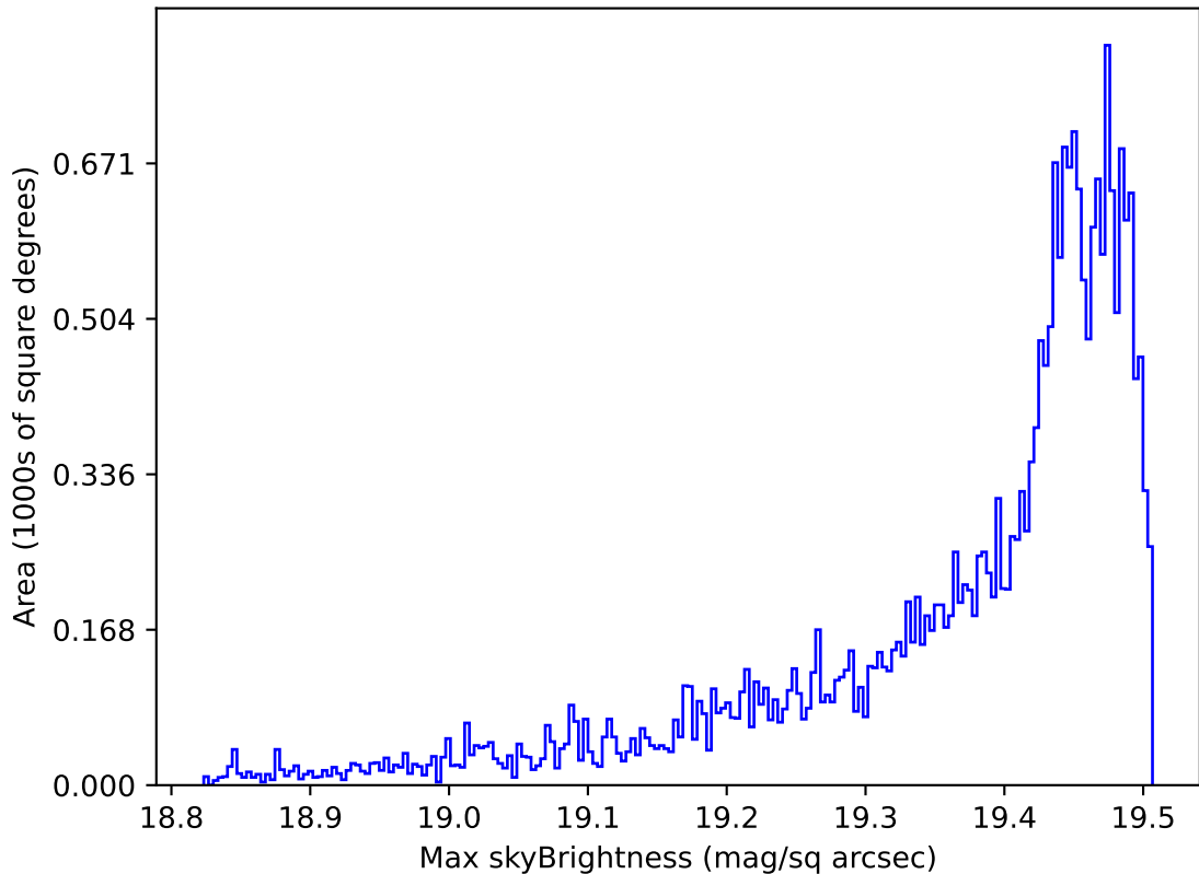
weather_cloudso36v3.4_10yrs All sky z band: Max skyBrightness
