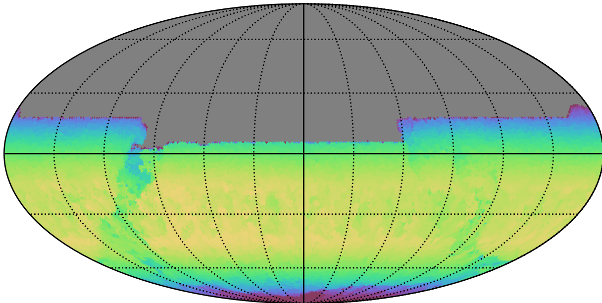
weather_cloudso36v3.4_10yrs All sky y band: Max skyBrightness
