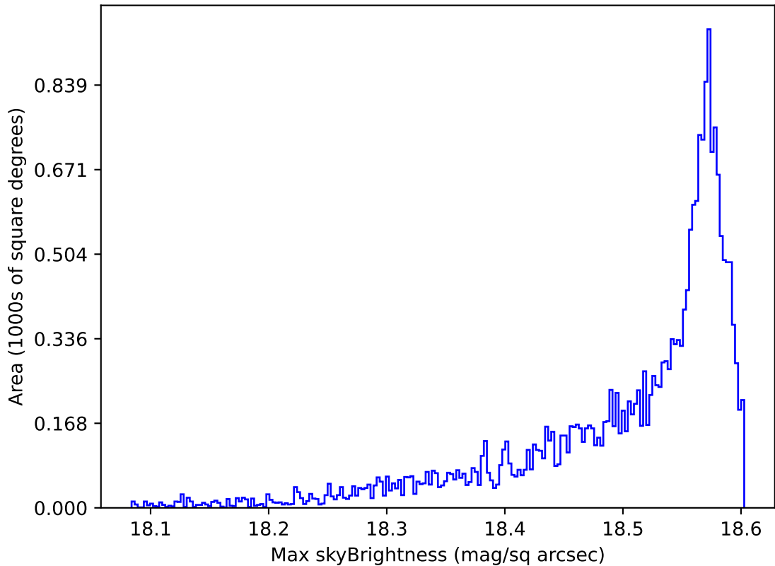
weather_cloudso36v3.4_10yrs All sky y band: Max skyBrightness
