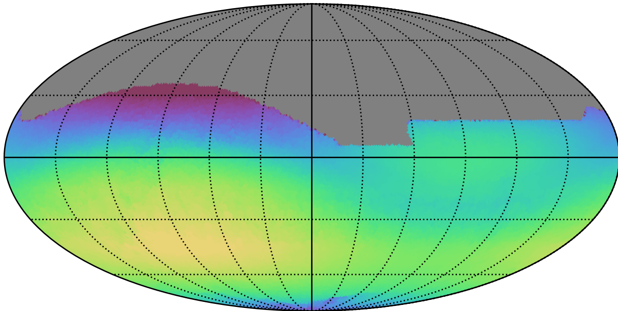
weather_cloudso36v3.4_10yrs All sky r band: Max skyBrightness
