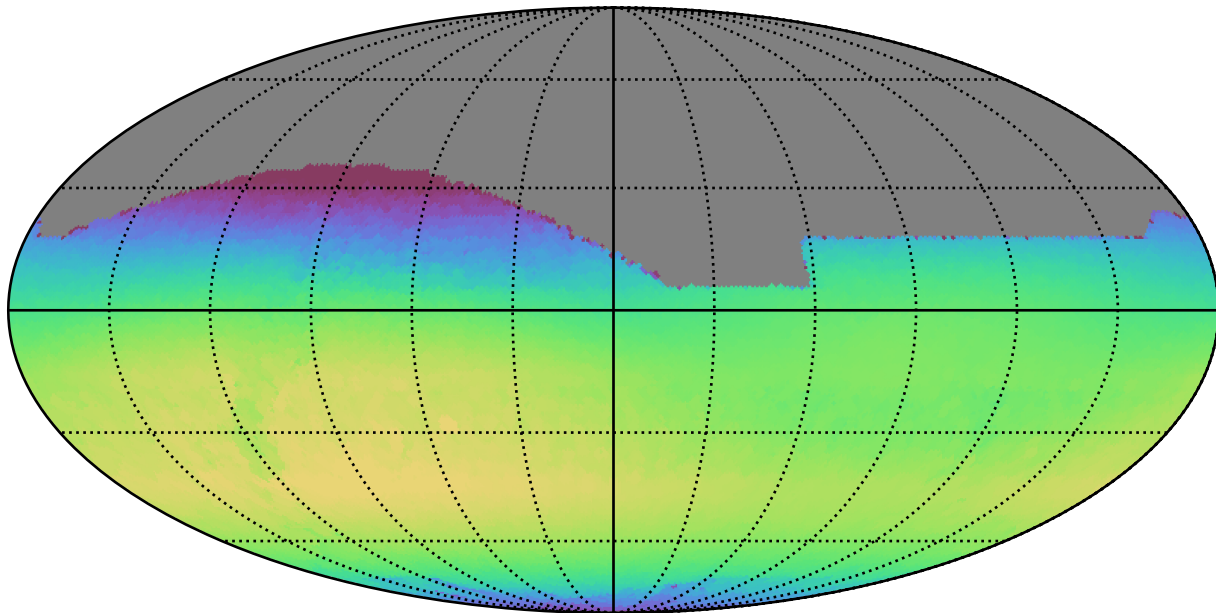
weather_cloudso36v3.4_10yrs All sky i band: Max skyBrightness
