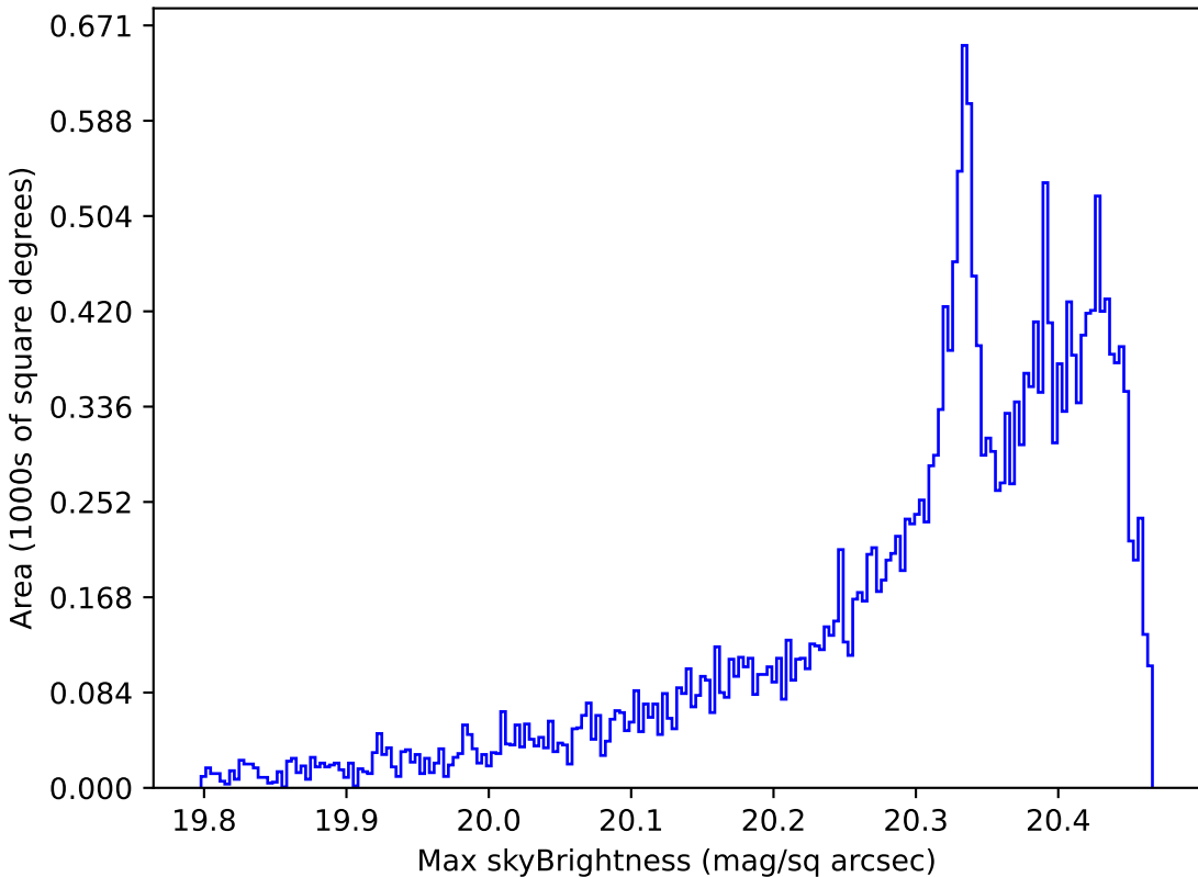
weather_cloudso36v3.4_10yrs All sky i band: Max skyBrightness
