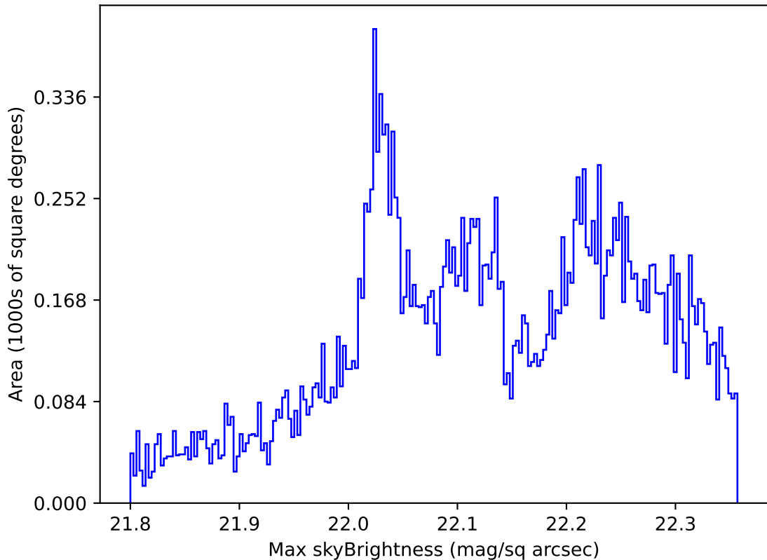
weather_cloudso36v3.4_10yrs All sky g band: Max skyBrightness
