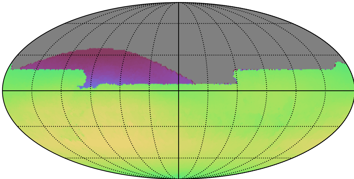
weather_cloudso36v3.4_10yrs All sky all bands: Max skyBrightness
