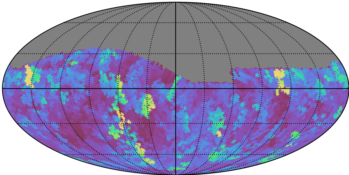
weather_cloudso36v3.4_10yrs Yr 1 z band: Max seeingGeom
