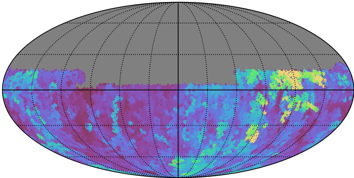
weather_cloudso36v3.4_10yrs Yr 1 u band: Max seeingGeom
