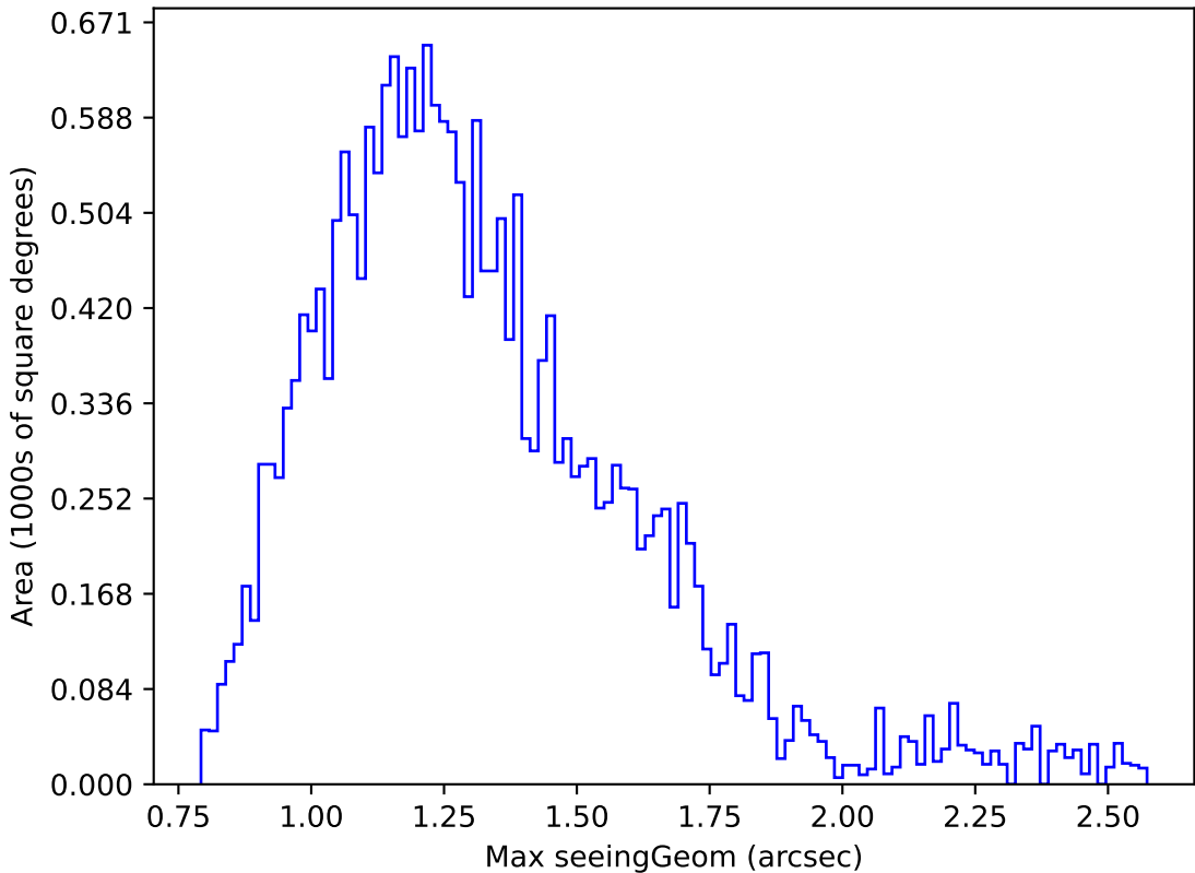
weather_cloudso36v3.4_10yrs Yr 1 u band: Max seeingGeom
