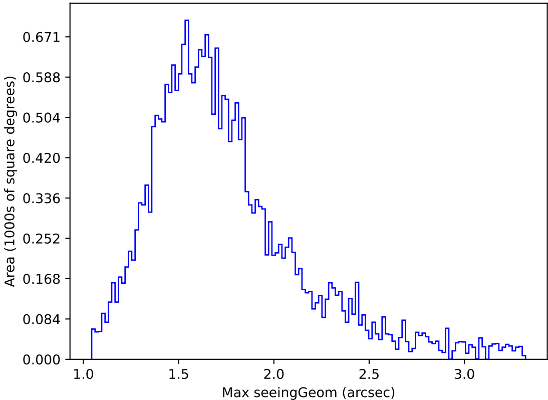
weather_cloudso36v3.4_10yrs Yr 1 all bands: Max seeingGeom
