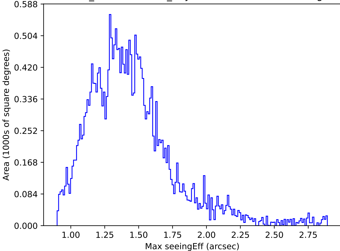
weather_cloudso36v3.4_10yrs Yr 1 z band: Max seeingEff
