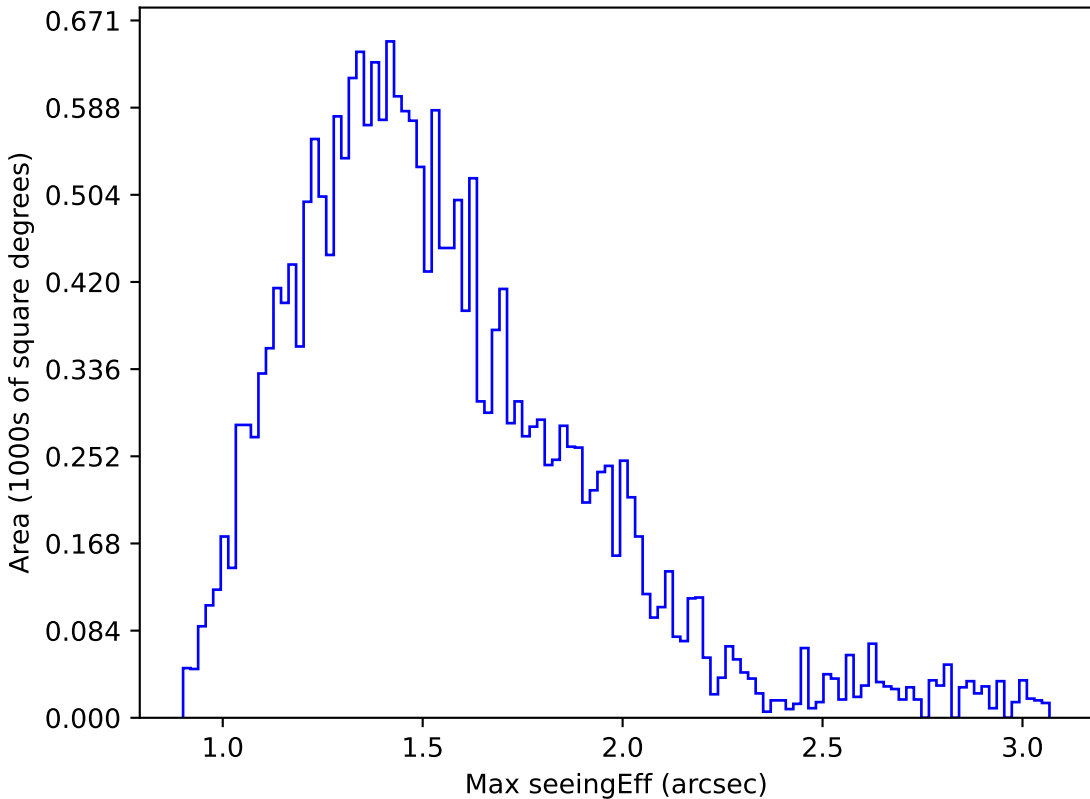
weather_cloudso36v3.4_10yrs Yr 1 u band: Max seeingEff
