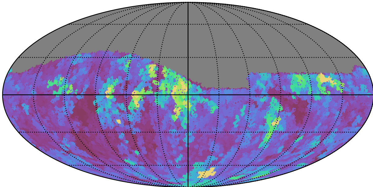
weather_cloudso36v3.4_10yrs Yr 1 r band: Max seeingEff
