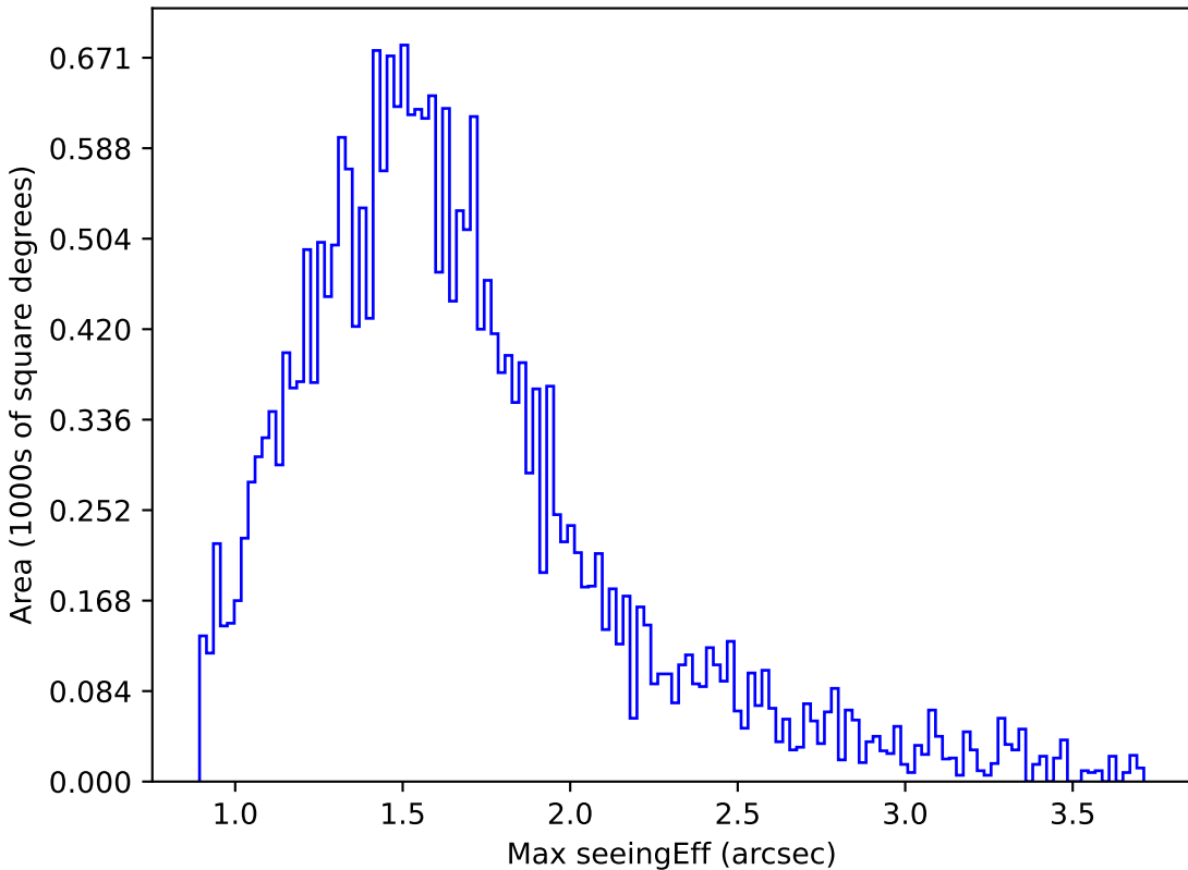
weather_cloudso36v3.4_10yrs Yr 1 r band: Max seeingEff
