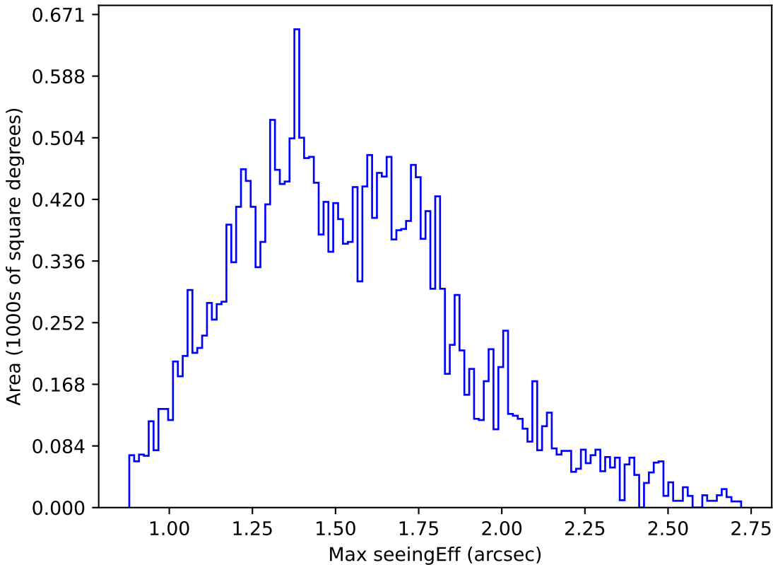
weather_cloudso36v3.4_10yrs Yr 1 i band: Max seeingEff
