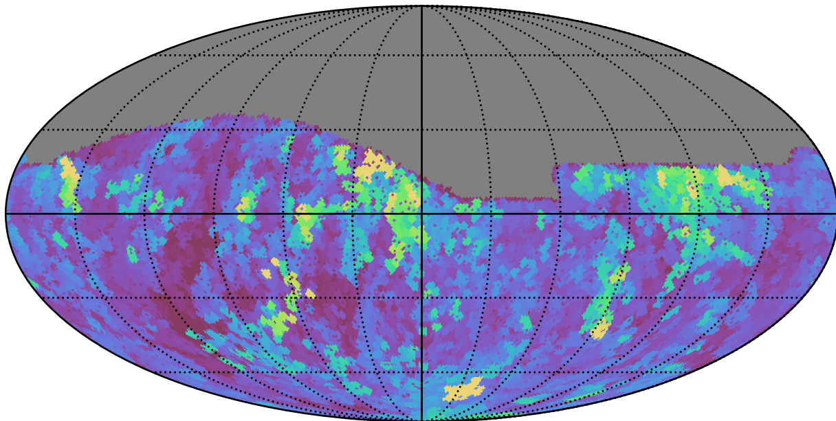
weather_cloudso36v3.4_10yrs Yr 1 all bands: Max seeingEff
