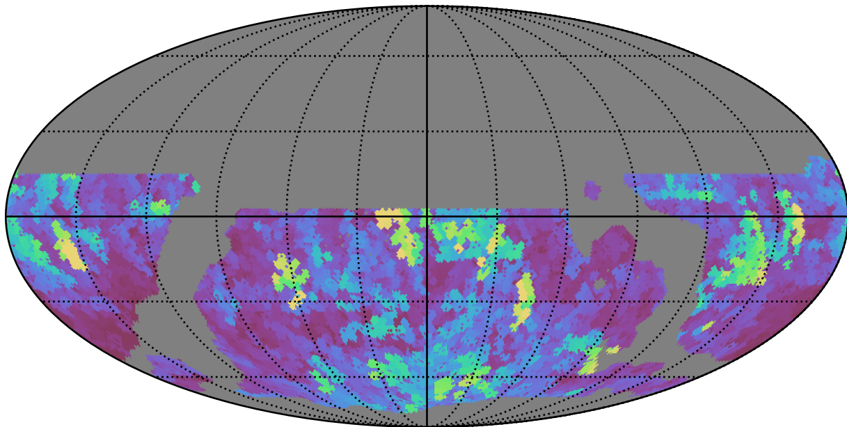
weather_cloudso36v3.4_10yrs WFD z band: Max seeingEff
