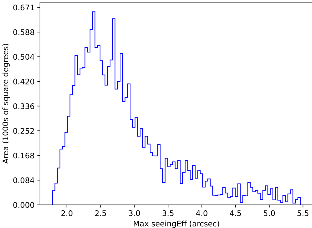
weather_cloudso36v3.4_10yrs WFD z band: Max seeingEff
