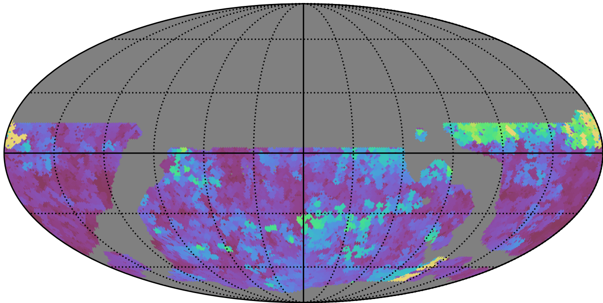
weather_cloudso36v3.4_10yrs WFD u band: Max seeingEff
