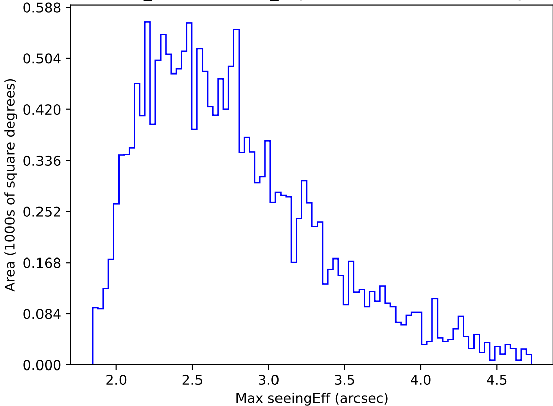
weather_cloudso36v3.4_10yrs WFD i band: Max seeingEff
