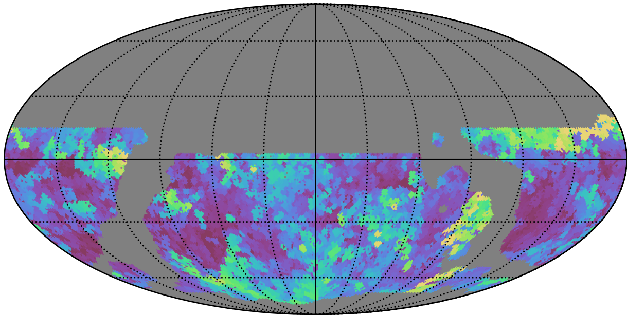
weather_cloudso36v3.4_10yrs WFD g band: Max seeingEff
