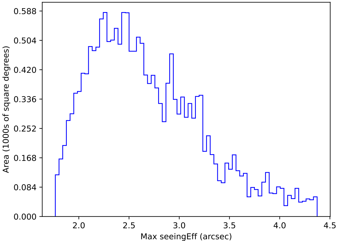
weather_cloudso36v3.4_10yrs WFD g band: Max seeingEff
