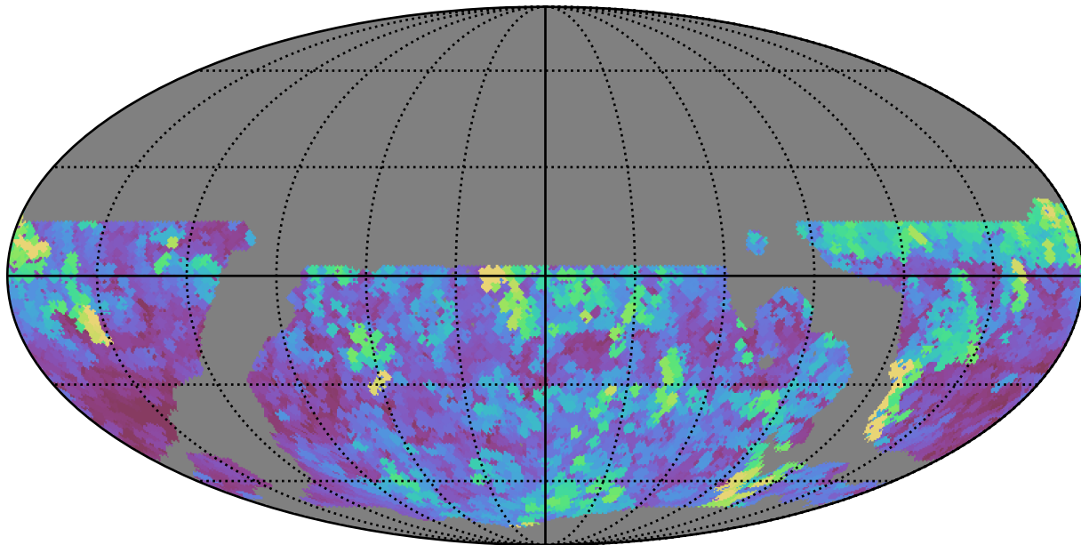
weather_cloudso36v3.4_10yrs WFD all bands: Max seeingEff
