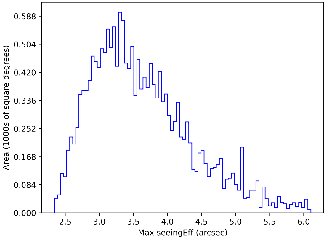
weather_cloudso36v3.4_10yrs WFD all bands: Max seeingEff
