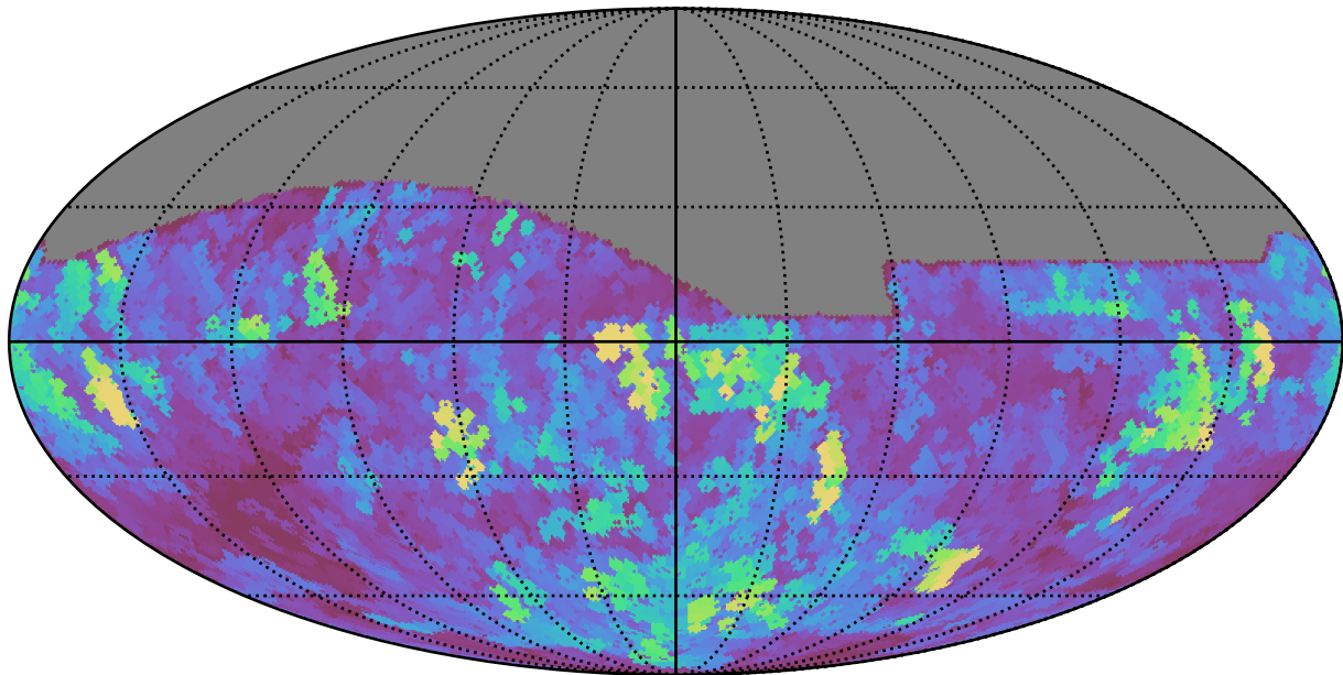
weather_cloudso36v3.4_10yrs All sky z band: Max seeingEff
