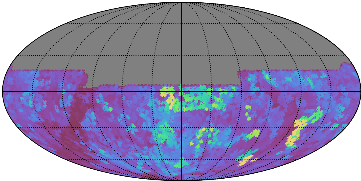
weather_cloudso36v3.4_10yrs All sky y band: Max seeingEff
